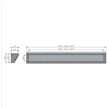
Tuscan G2 60 Drawing
