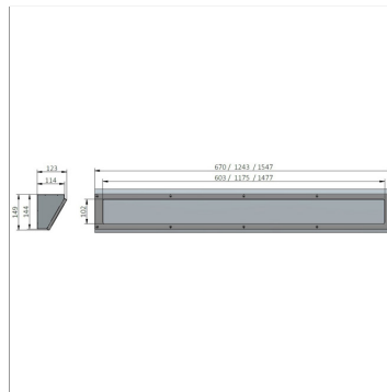
Tuscan G2 60 Blank Ends Option Drawing
